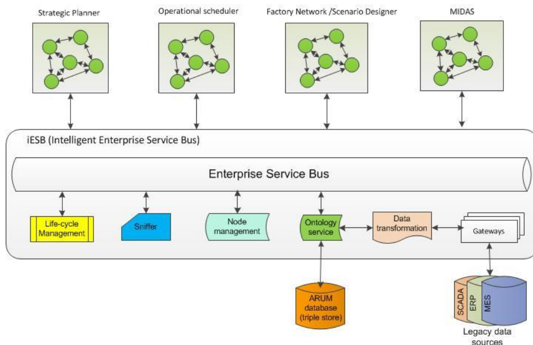
Figure 5: Integration of MAS and SOA using an Enterprise Service Bus
