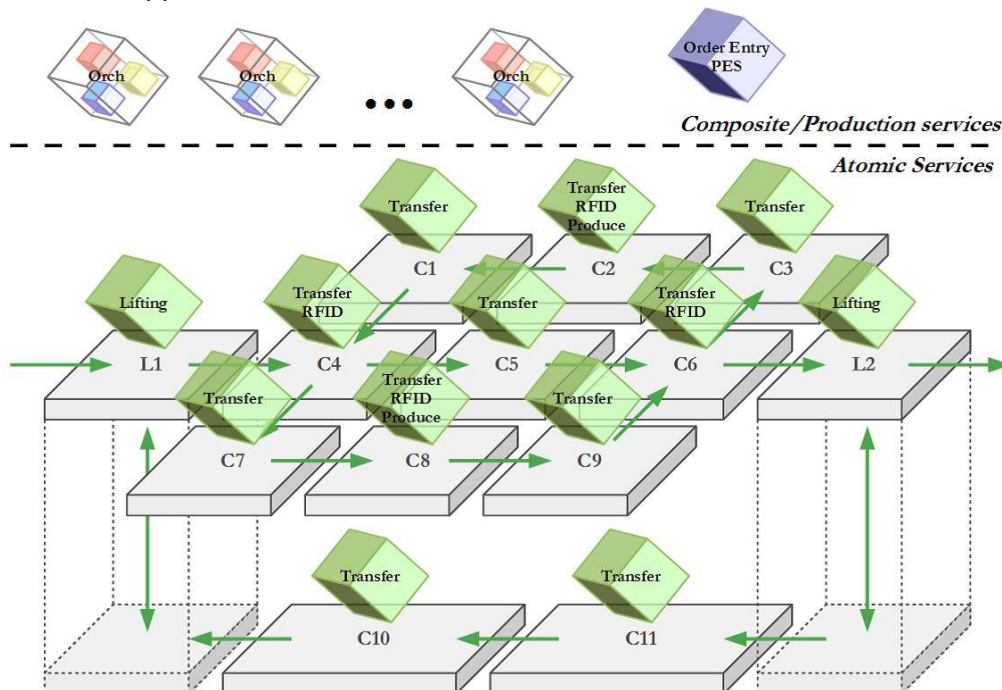
Figure 10: Service landscape of the automation system
