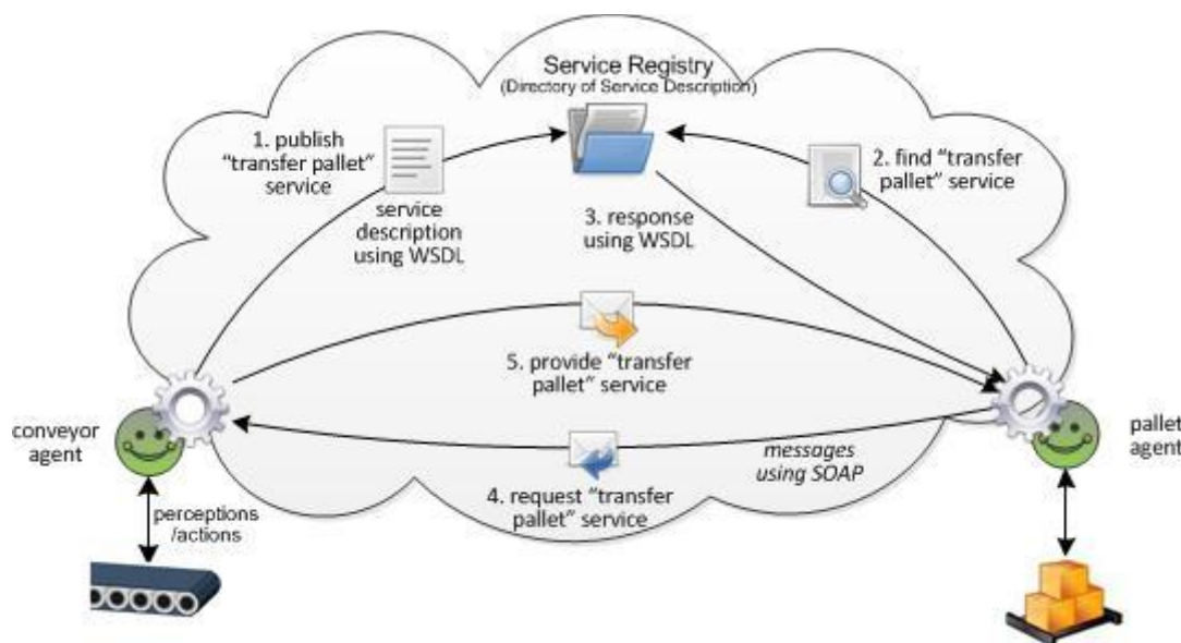
Figure 4: Example of a service-oriented multi-agent system
