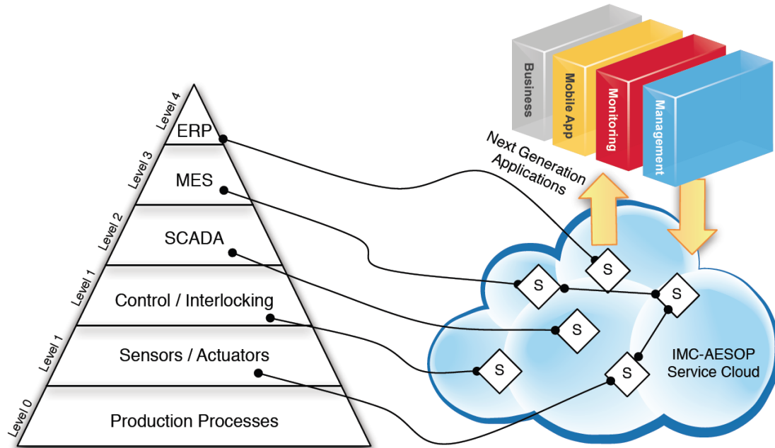
Figure 2: Industrial automation evolution: complementing the traditional ISA-95 automation world view (pyramid on the left side) with a flat information-based infrastructure for dynamically composable services and applications (right side)
