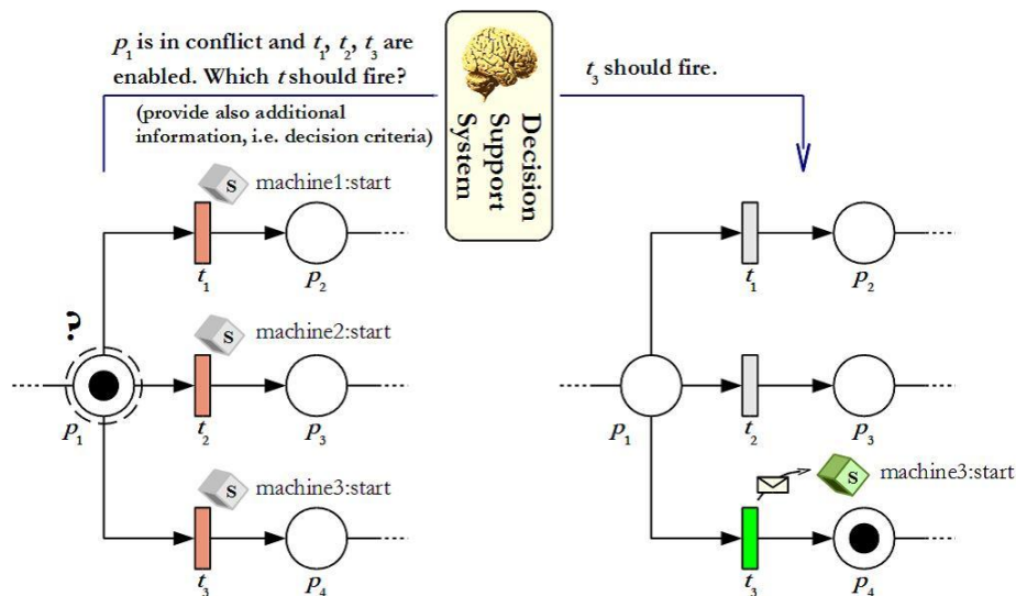
Figure 12: Petri net based orchestration with decision support system
