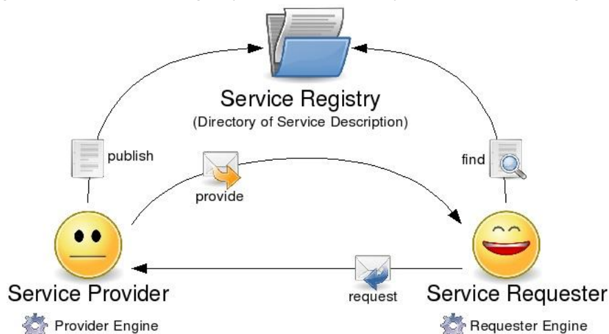
Figure 1: SOA concepts
