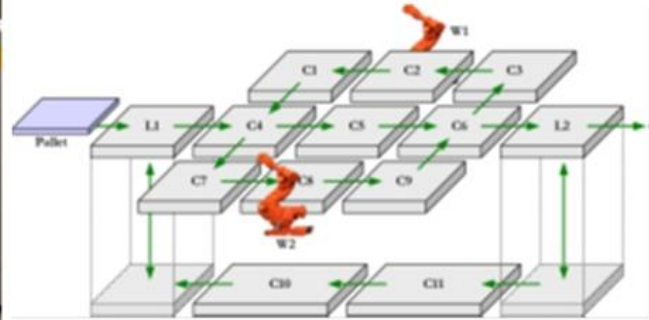
Figure 8: Prodatec/FlexLink DAS 30 used for the demonstration (located at Schneider Electric Automation GmbH in Seligenstadt, Germany)
