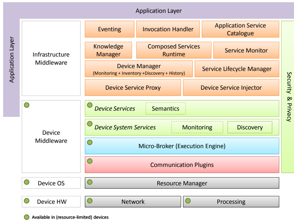
Fig. 1. UICO Reference Architecture. A minimal device middleware enables the ad-hoc cooperation of objects whose capabilities can be enhanced with an infrastructure middleware when available. This enables uniform support for a broad spectrum of application scenarios while being suitable for resource-constrained embedded systems. Security and privacy are cross-cutting concerns that must be handled at both infrastructure and device middleware levels in an adequate manner.
