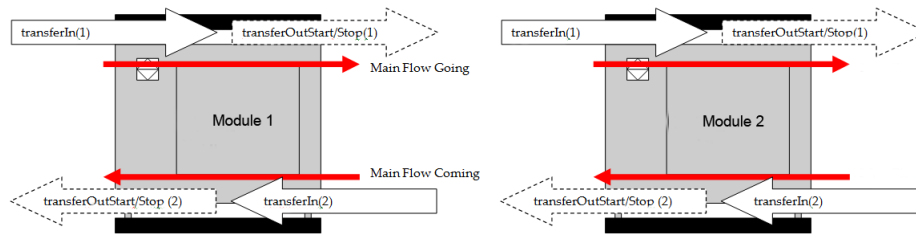
Fig. 2. Example of device-only collaboration in the automation domain. Two modular material handling units can collaborate and negotiate during runtime the transfer of a pallet thanks to a well-defined communication interface based on Web Services. This provides a new way for material handling units from different manufacturers (heterogeneous) to collaborate without a prior knowledge of each other.
