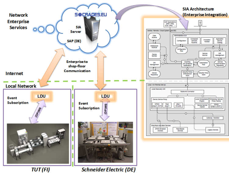
Fig. 3. Example of device collaboration assisted by the infrastructure. Devices at the same site cooperate with each other either directly or via their surrounding infrastructure. Multiple local infrastructures may cooperate to optimize the resource utilization. A local discovery unit enables the interaction between devices at different sites via an enterprise Intranet or via the Internet.
