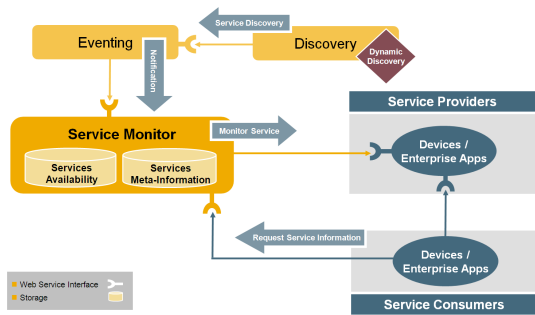
Figure 7. Service Monitor
