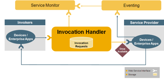
Figure 4. Invocation Handler
