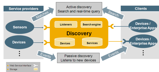
Figure 9. Device Discovery
